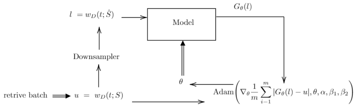
Figure A.1: The training process for the AudioEDSR. The double lined arrows mark the start of a new cycle
