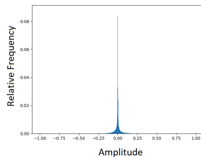
Figure 3.10: A graph showing the distribution of amplitudes from a sample the VCTK dataset
