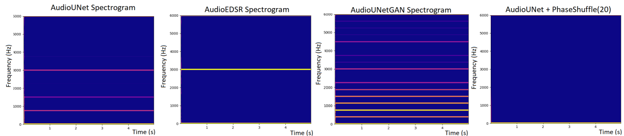
Figure 4.4: Spectrograms showing the tonal artifacts produced by the x upsampling layer of the three Deep learning models when the input is an empty signal. The image also shows how modifying the network with phase shuffles can reduce these artifacts.
